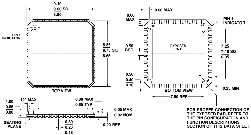
COMPLIANT TO JEDEC STANDARDS MO-220-VMM4 Figure 67. 64-Lead Lead Frame Chip Scale Package [LFCSP_VQ] 9 mm × 9 mm Body, Very Thin Quad (CP-64-3) Dimensions shown in millimeters
