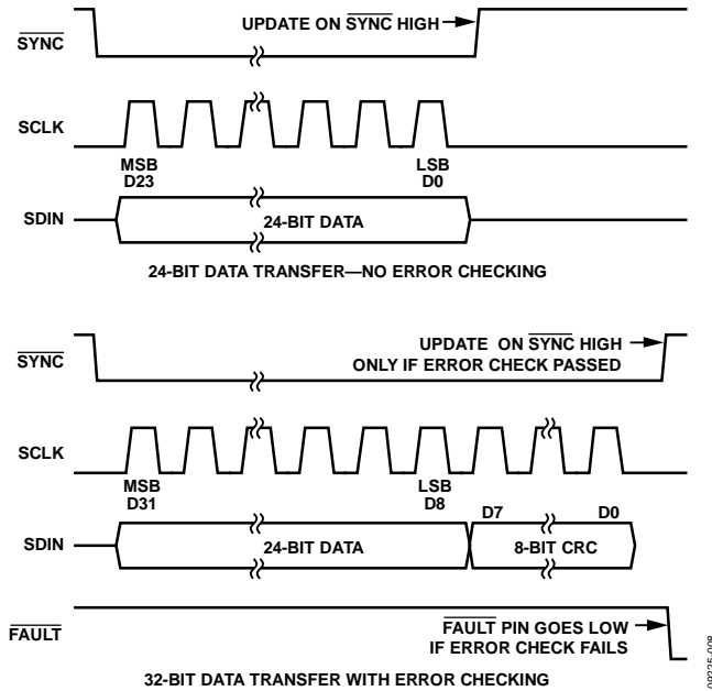
Figure 54. PEC Timing
