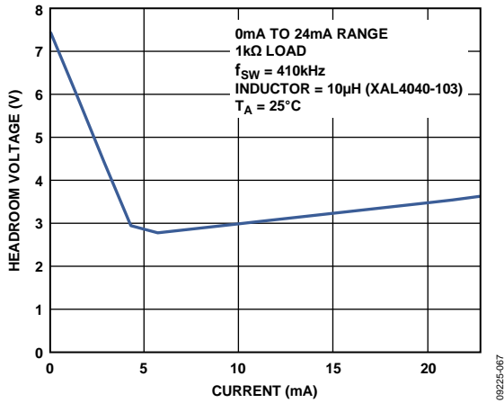
Figure 31. DC-to-DC Converter Headroom vs. Output Current (See Figure 56)
