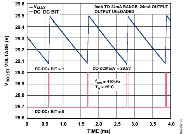
Figure 57. Operation on Reaching V_{\text{MAX}}
