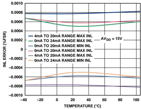
Figure 11. Integral Nonlinearity vs. Temperature, Internal R_{SET}
