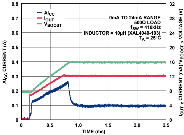
Figure 60. Al CC Current vs. Time for 24 mA Step Through 500 Ω Load with External 51 kΩ Compensation Resistor
