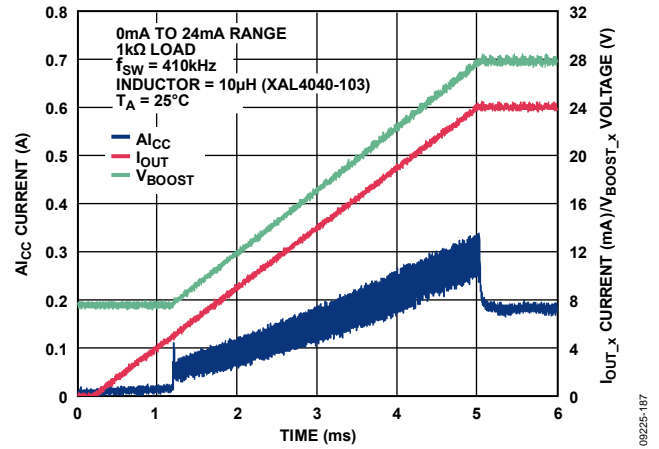
Figure 61. Al CC Current vs. Time for 24 mA Step Through 1 kΩ Load with Slew Rate Control
