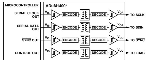
Figure 65. Isolated Interface
