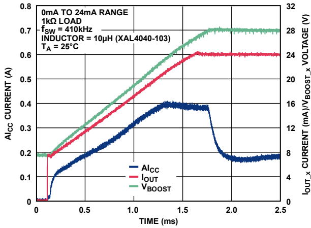
Figure 59. Al CC Current vs. Time for 24 mA Step Through 1 kΩ Load with External 51 kΩ Compensation Resistor
